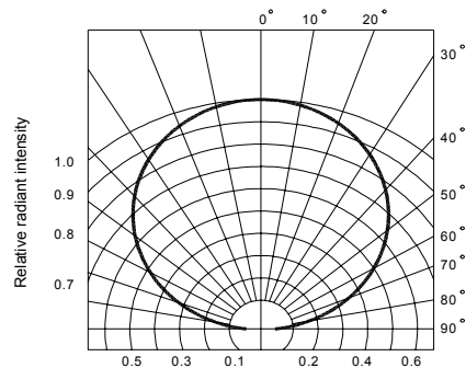
Fig.6 Radiation diagram
